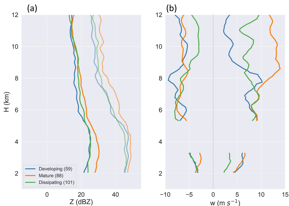
Figure 9. Profiles of (a) the average (darker lines) and maximum reflectivity (Z) and (b) 95th percentiles of updrafts with w > 1 \text{ m s}^{-1} and downdrafts with w < -1 \text{ m s}^{-1} for developing, mature, and dissipating DCCs.
