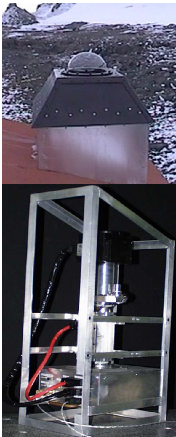
Figure 1. Glass dome at the roof of Punta Plaza shelter (top) used to house the FotAntar-1 instrument (bottom).
