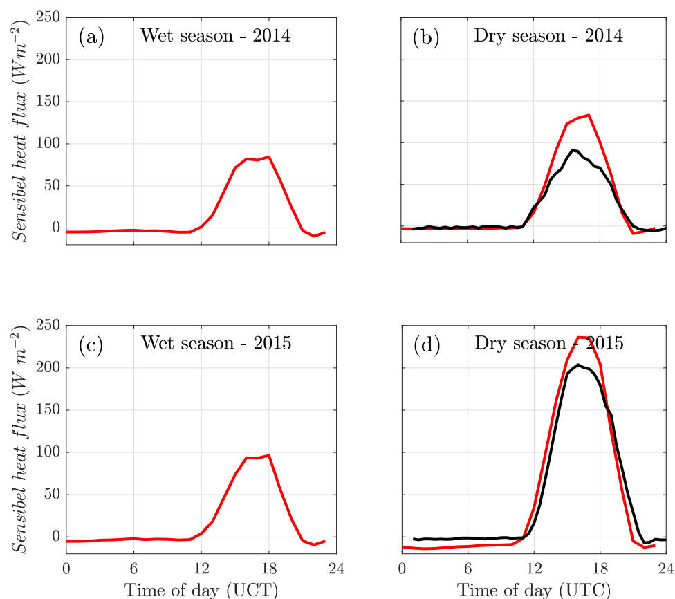
Figure 5. Sensible heat flux values through experimental data (black line) and ERA5 (red line) at the T3 site. The data correspond to the wet seasons of (a,c) 2014 and 2015, and the dry seasons of (b,d) 2014 and 2015.
