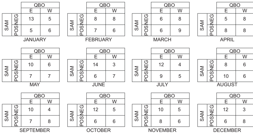
Fig. 3. Monthly contingency tables between the QBO and SAM indices. SAM index (filtered) calculated for 700 hPa. The upper-left square corresponds to the events of the negative SAM phase during the easterly QBO phase (E); the upper-right square corresponds to the cases of negative SAM phase during the westerly QBO (W); the bottom-left square corresponds to events of positive SAM phase along easterly QBO (E); and the bottom-right square corresponds to occurrences of a positive SAM phase along westerly QBO (W).
