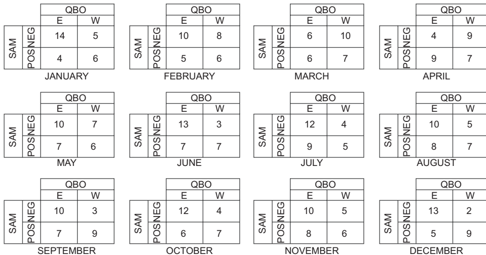
Fig. 4. Same as Figure 3, but for SAM index calculated at 200 hPa.
