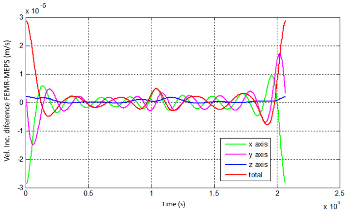
Figure 6.9 - Spacecraft's velocity increment difference Bacchus i=0 degrees.
