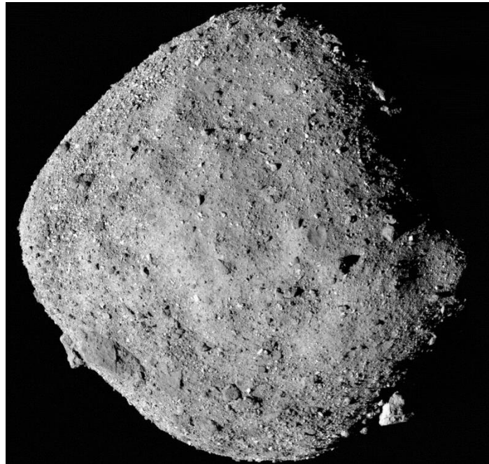
Figure 5.1 - Asteroid Bennu.
