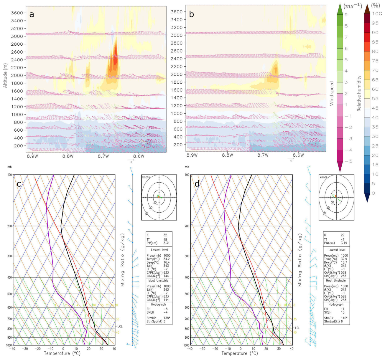
Figure 10 - Relative humidity (%) and horizontal and vertical wind (m s -1 ) in the Alcácer do Sal region a) with fire and b) without fire. State curves and evolution in Skew-T Log-p nomograms in the Alcácer do Sal region on 28th July 2010, simulated by BRAMS-SFIRE at latitude 38.33° N and longitude 8.75° W c) with fire and d) without fire.
