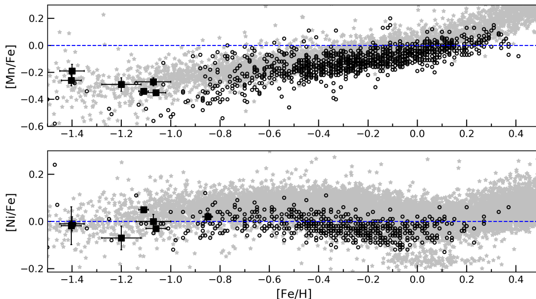
Fig. 10. Mean abundance ratio of the Fe-peak elements Mn (top) and Ni (bottom) for each of our clusters (filled squares with error bars), compared with APOGEE bulge stars (asterisks - Rojas-Arriagada et al. 2020) and the general trend of disk/halo stars (circles- Reddy et al. 2003, 2006; Battistini & Bensby 2015; Lomaeva et al. 2019). Our BGCs generally follow the bulge field-star trend.
