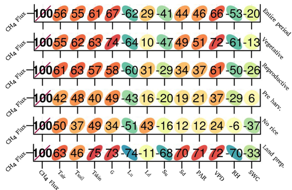
Figure 3. Correlation coefficient matrixes (in percentage) using lattice between the half-hour CH 4 fluxes and atmospheric and soil variables for the vegetative, reproductive, pre-harvest, no rice, and land preparation periods. A perfect positive correlation is presented as a 45-degree line, positive slope, red color, and a value of 100. The absence of correlation has a circular shape, light color, and a value of zero. A perfect negative correlation is presented as a -45-degree line, negative slope, blue color, and a value of -100.
