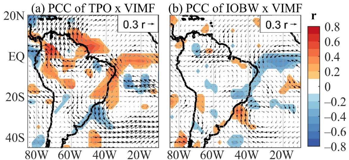
Figure 7. Partial correlations for the vertically integrated moisture flux (VIMF) components and their divergence (shades) during summer of the (a) TPO and VIMF; (b) IOBW and VIMF. Shades encompass significant correlations at a 95% confidence level using Student’s t -test. Vectors indicate the correlations with the VIMF components. Arrow in the right-lower corner gives the vector base magnitude in correlation units. Bold arrows indicate vectors when at least one component has significant correlation at a 95% confidence level.
