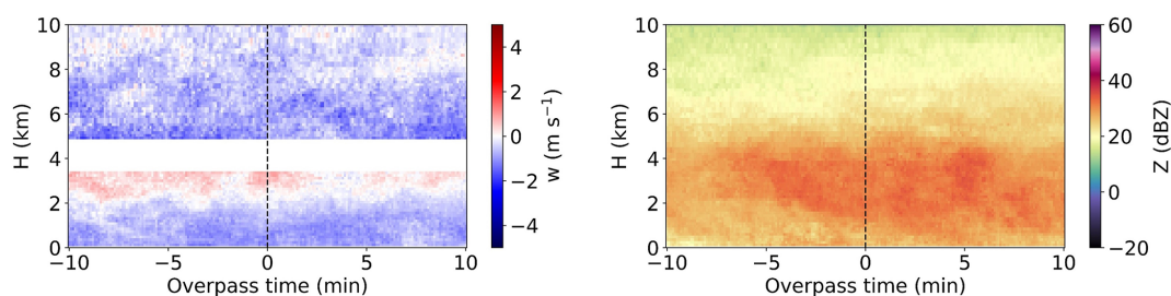
Figure 12. Time–height composites of vertical velocity ( w ) and reflectivity ( Z ) from the RWP for DCCs in the “mature” lifecycle stage. (For each pixel, the composites represent the median value across all DCCs classified as “mature”.)
