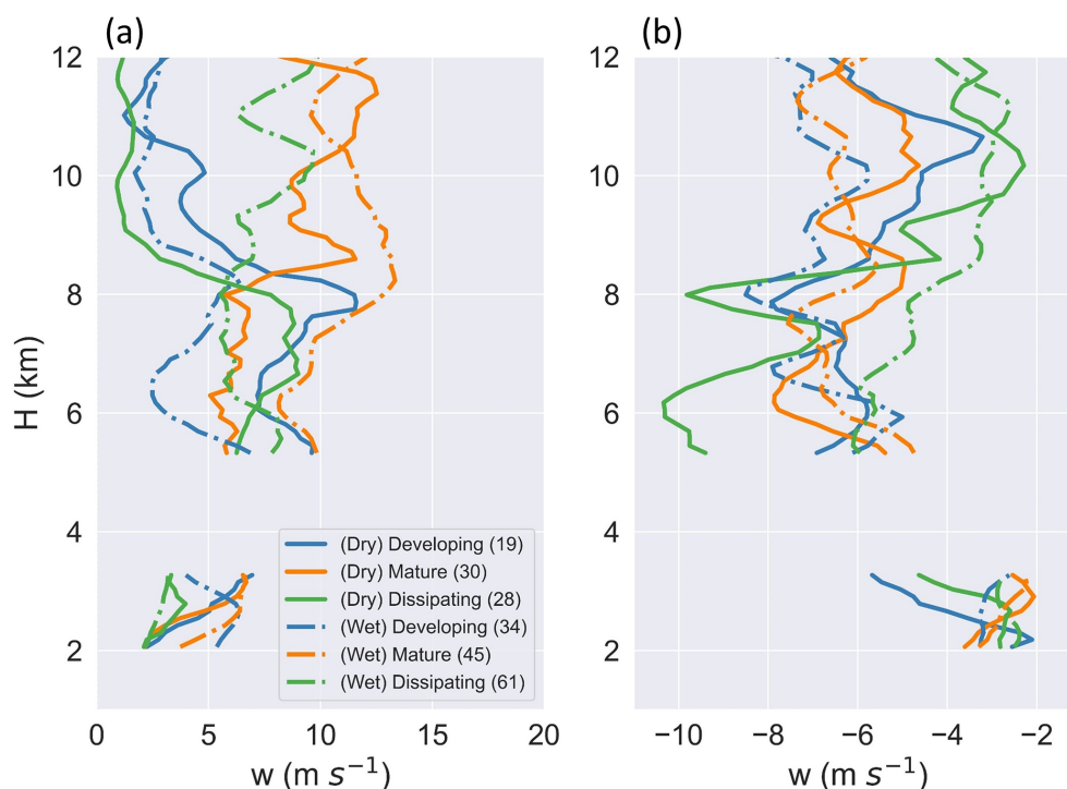
Figure 11. Profiles of (a) strongest updrafts (95th percentile of w > 1 m s -1 ) and (b) strongest downdrafts (5th percentile of w < -1 m s -1 ) for developing, mature, and dissipating DCCs from the dry season (solid lines) and wet season (dotted–dashed lines).
