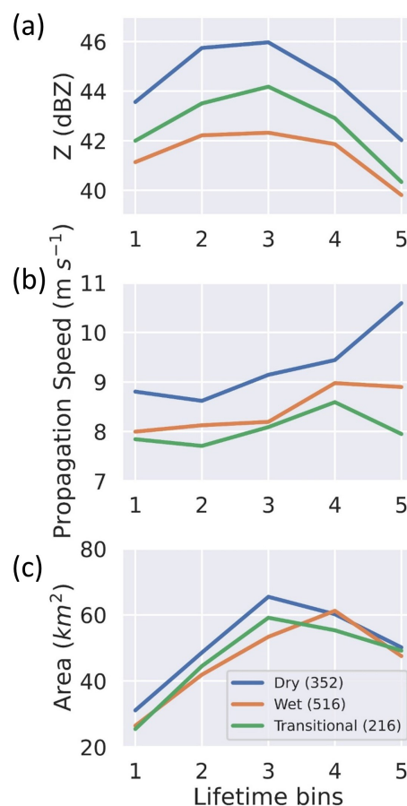
Figure 7. Trends in average Z , propagation speed, and area over the DCC lifetime for cells classified by seasons and observed within 20 km of MAO with lifetime > 36 min, propagation speed > 0.5 m s -1 , and A < 500 km 2 . The number of cells is listed in the legend.
