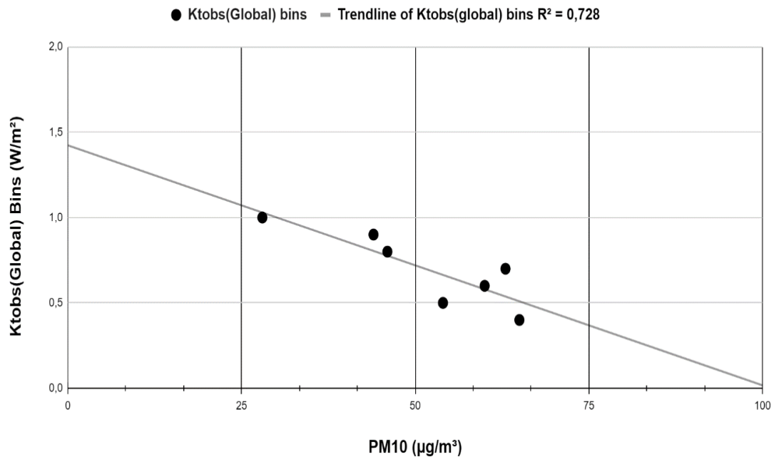
Behavior of Ktobs(global) for the Rainy Season in terms of PM10
