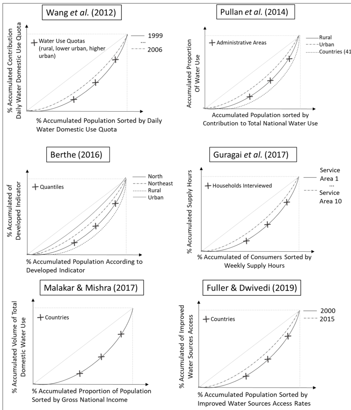
Figura 2.8 – Curvas de Lorenz adaptadas por Wang et al. (2012), Pullan et al. (2014), Berthe (2016), Guragai et al. (2017), Malakar e Mishra (2017) e Fuller e Dwivedi (2019).
