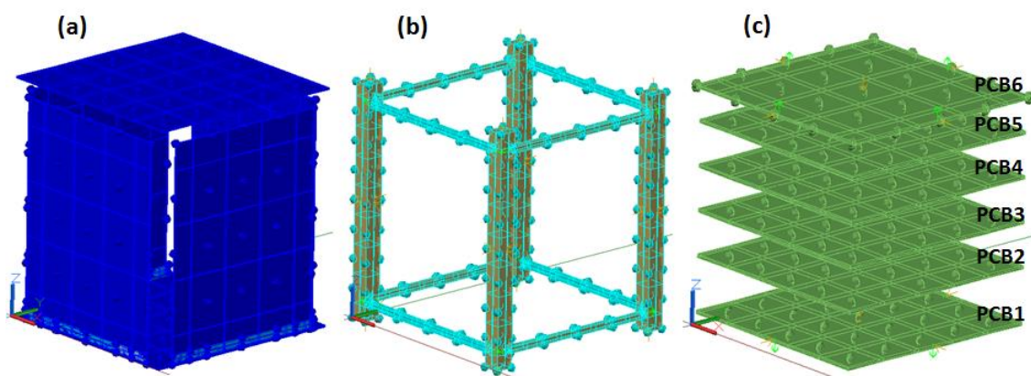
(a) Face (b) Estrutura (c) PBC.
