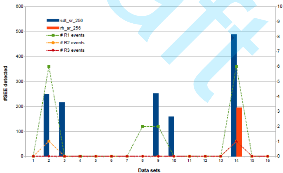
Figure 9: The NANOSATC-BR1 SEE tolerance comparison of two shift-registers (256 stages, 8 inverters) (Medeiros et al., 2014; Noval et al., 2016).
