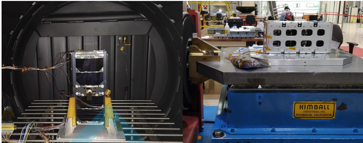
Figure 4: The NANOSATC-BR2 mounted with several internal and external thermocouples inside the Thermal Vacuum Chamber (left), and the CubeSat placed inside a Test-POD on a shaker at the Integration and Tests Laboratory – LIT / INPE - MCTI (right) (Asencio, 2021).
