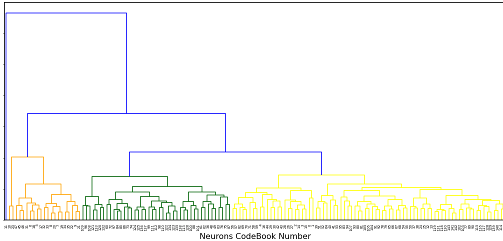
Figure 2.5 - Dendrogram Results.
