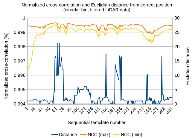
Fig. 8. Position estimation errors of the template matching algorithm (blue) and respective NCC values, highest (orange) and lowest (yellow).
