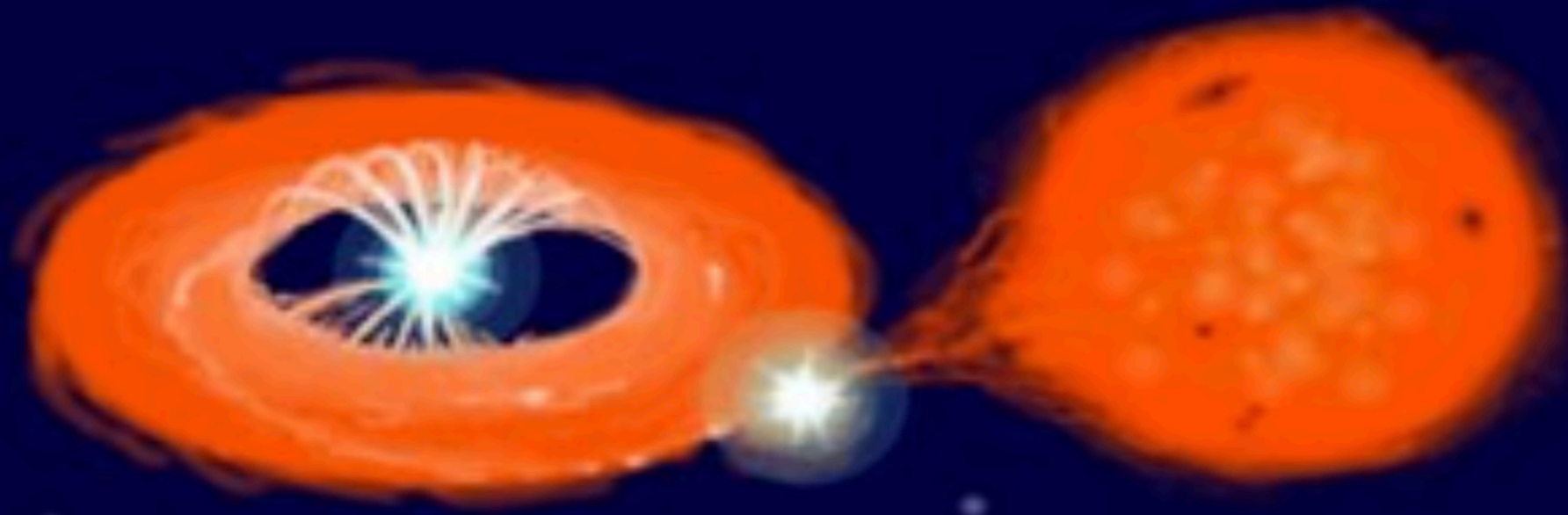
Intermediate polar
