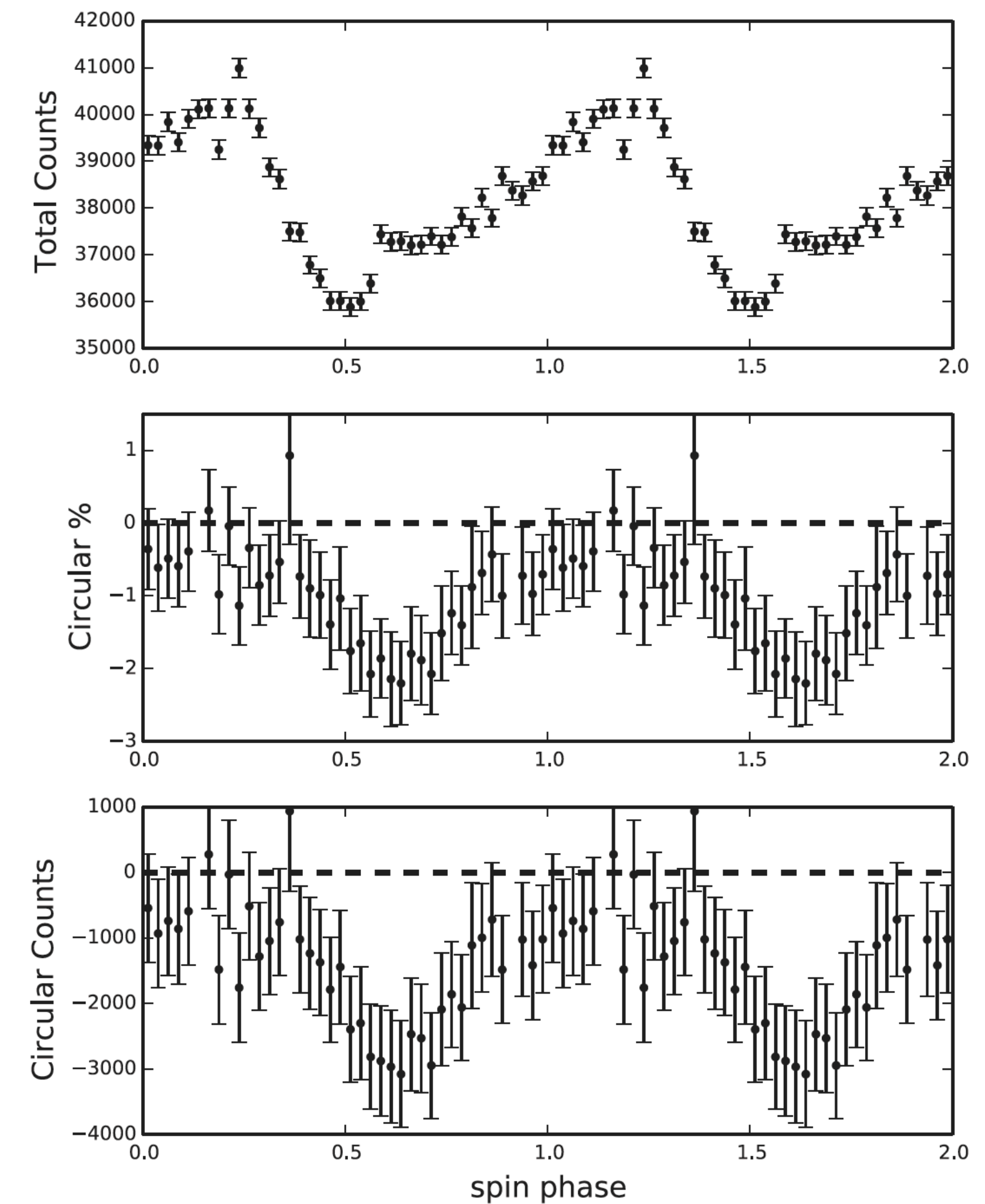
Figure 3. Spin-folded photometry and circular polarimetry of the June 25 observations. Bin sizes correspond to \sim 46 s (0.025 spin-phase bins) for the photometry and polarimetry.
