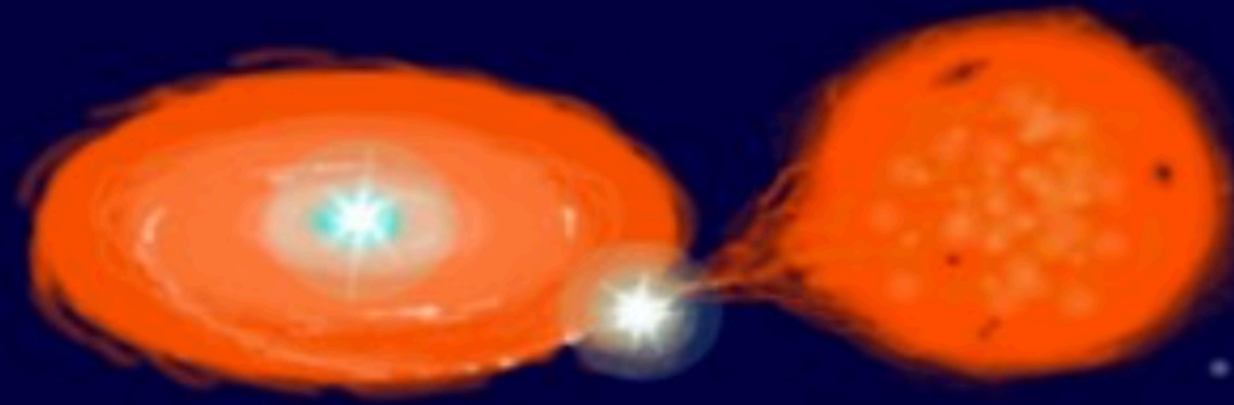
Non-magnetic CV
