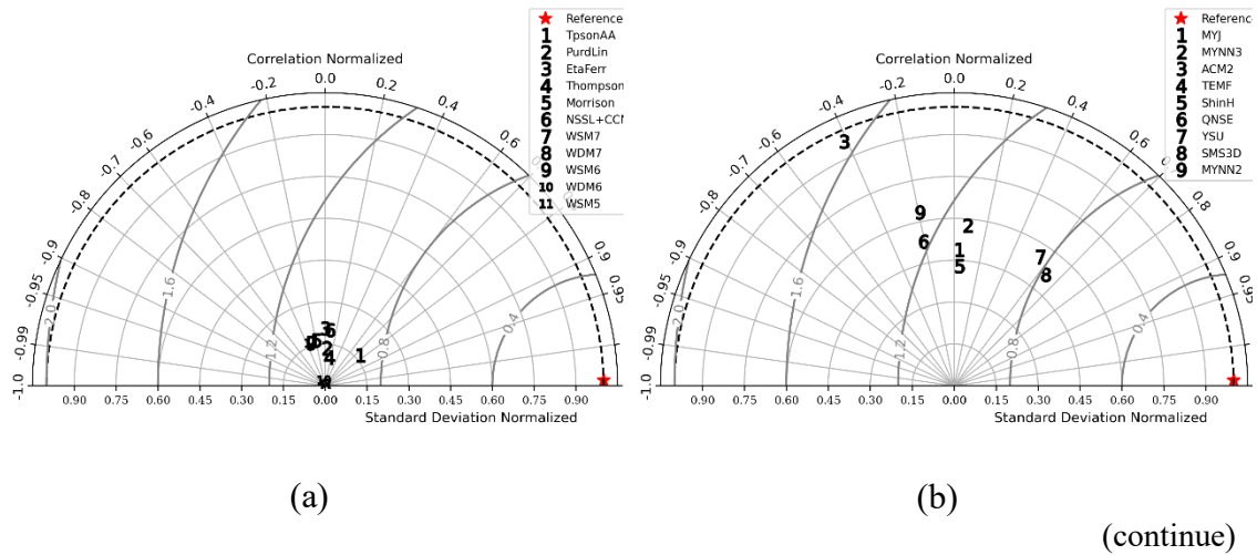
Figure 5.7 – Taylor diagram for event 2 settings.
