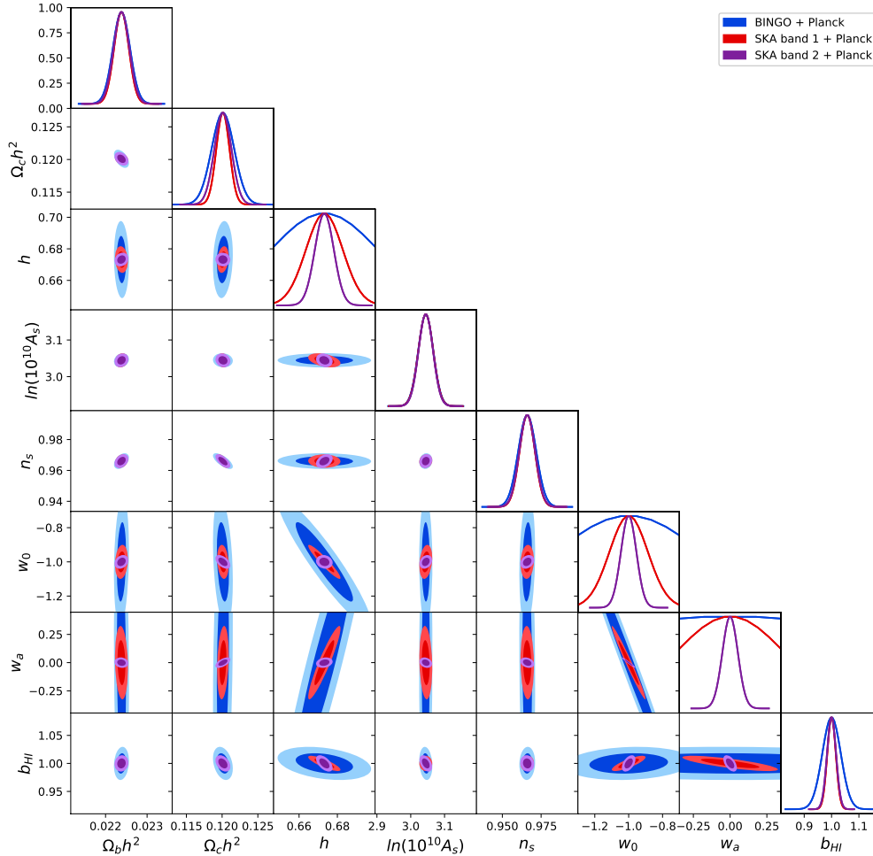
Fig. 13. One- and two-dimensional (68% and 95% CL) cosmological constraints for a CPL parameterization from BINGO, SKA1-MID band 1, and SKA1-MID band 2 in combination with Planck data. This illustrates that BINGO can be considered a pathfinder for constraints obtained by SKA.
