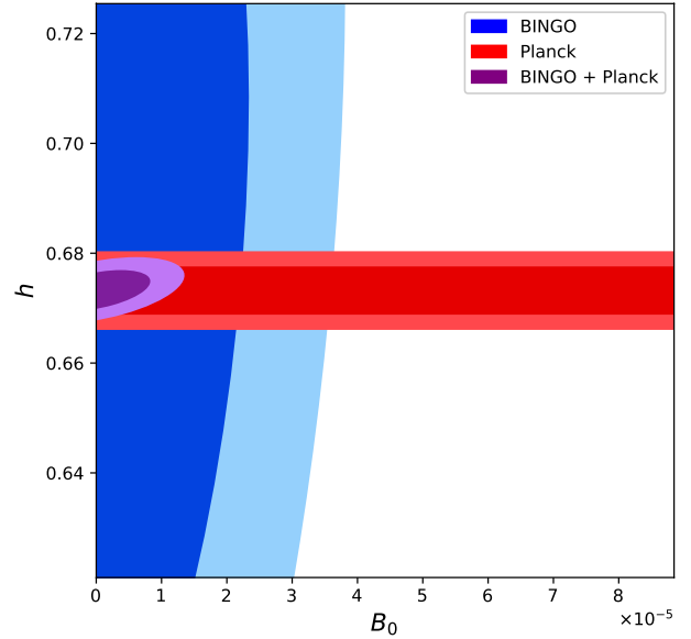
Fig. 14. Marginalized constraints (68% and 95%) CL on the modified gravity parameter B_0 and the Hubble parameter from BINGO, Planck , and BINGO + Planck .
