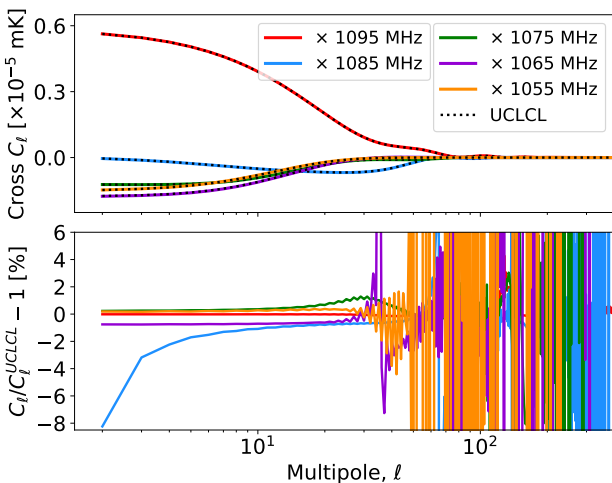
Fig. A.2. Same as Fig. A.1, but for the cross-correlation C_\ell^{ij} s ( i \neq j ) between the frequency bin centered at 1105 MHz ( z = 0.28 ) and the five following frequency bins, with bandwidth of 10 MHz.
