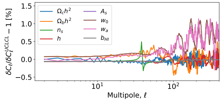
Fig. A.4. Percentage relative difference comparing the derivatives, \delta C_\ell^{ij} = dC_\ell^{ij}/dx (for auto-correlation, i = j ), with x representing each cosmological and 21 cm parameter, calculated in this work and by using the UCLCL code. All the cases correspond to a frequency channel with a bandwidth of 10 MHz centered at 1110 MHz.
