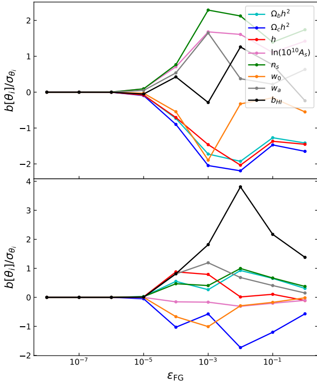
Fig. 11. Ratio of bias to the marginalized statistical errors for each parameter as a function of the residual foreground contamination amplitude, \epsilon_{FG} , from BINGO ( top ) and BINGO + Planck ( bottom ).
