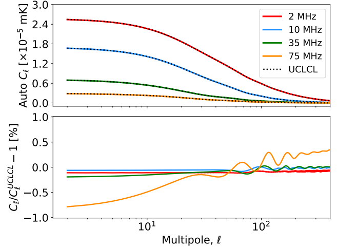
Fig. A.3. Comparison between the auto-correlation C_\ell^{ij} s calculated in this work and using the UCLCL code for four different bandwidths between 2 and 75 MHz, all of them centered at a frequency of 1110 MHz. Again, the upper panel shows the results overplotted and the lower panel shows the percentage difference among them.
