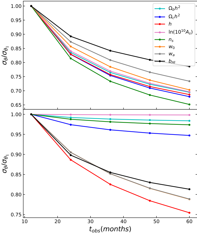
Fig. 5. Constraints on the cosmological and HI parameters as a function of the total observational time relative to those with t_{\text{obs}} = 1 year for BINGO ( top ) and BINGO + Planck ( bottom ). We vary t_{\text{obs}} in a range of [1, 2, 3, 4, 5] years. In the bottom plot w_a is on top of w_0 , which cannot be seen.
