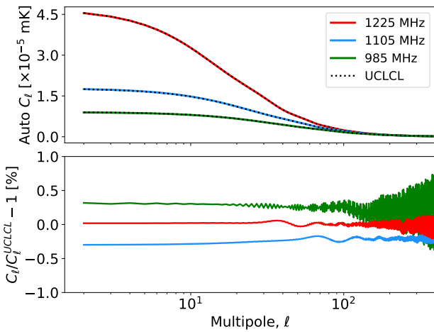
Fig. A.1. Comparison between the auto-correlation C_\ell^{ij} s (for i = j ) calculated in this work and those obtained with the UCLCL code at three BINGO redshift bins, centered at the frequencies 985, 1105, and 1225 MHz (redshifts z \approx 0.44, 0.28 , and 0.16 , respectively), and bandwidths of 10 MHz. The upper panel shows the UCLCL results overplotted as dotted lines on each of the calculated curves (colored lines), while the lower panel shows the percentage relative difference among them.
