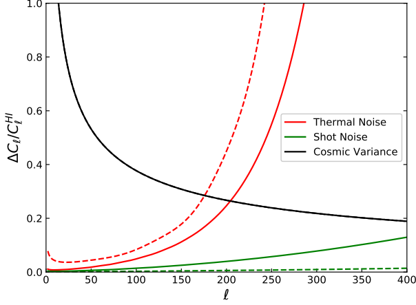
Fig. 2. Fractional uncertainties expected for the angular power spectrum for the BINGO experiment ( f_{\text{sky}} = 0.07 ) for redshifts z = 0.127 (solid lines) and z = 0.449 (dashed lines) after 1 year of sky integration. The ratio is plotted between different sources of uncertainty (cosmic variance, shot noise, and thermal noise) and the HI angular power spectrum, \Delta C_\ell / C_\ell^{\text{HI}} , as a function of multipole. For the cosmic variance the standard formula, \sqrt{2/(2\ell + 1)} f_{\text{sky}} , is used, and for the thermal and shot noise \Delta C_\ell is equal to their angular power spectrum multiplied by the cosmic variance factor.
