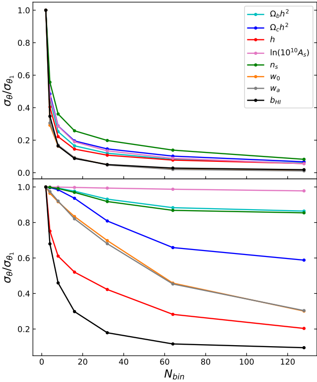
Fig. 7. Projected constraints on the cosmological and HI parameters as a function of the number of bins for BINGO ( top ) and BINGO + Planck ( bottom ). They show that w_0 , w_a , and h can have their constraints further improved for N_{\text{bin}} > 30 .
