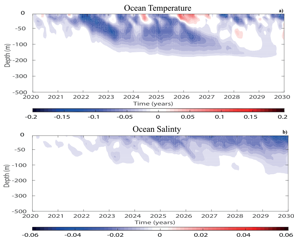
Figure 4. Time x depth (0–500 m) mean profile of (a) ocean temperature and (b) salinity differences ( layer_{max} - layer_{ctl} ) from the spatial average in the TAO domain ( 30^{\circ}\text{S} - 30^{\circ}\text{N} ), during the 10 years of model simulation (July 2020–June 2030).
