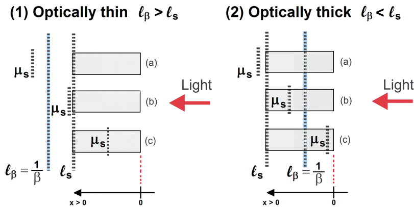
FIG. 6. Optically thin and thick regimes depending on the thermal diffusion length ( \mu_s ), the light penetration depth ( \ell_\beta ), and the sample thickness ( \ell_s ).
