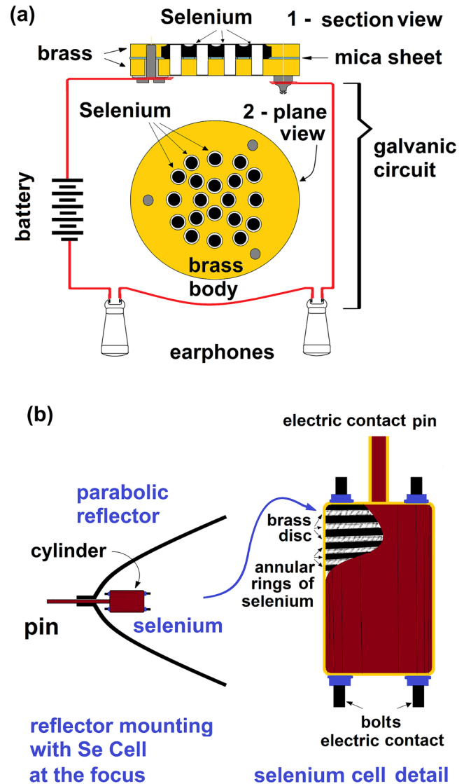
FIG. 1. Two types of selenium cells: (a) a disk form to be used at the lens focus and (b) a cylinder form to be used in a parabolic reflector mirror with the selenium cell at its focus. Adapted from Refs. 11 and 12.
