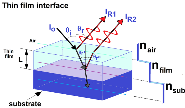
FIG. 11. Multireflection waves in a thin film deposited over a substrate.
