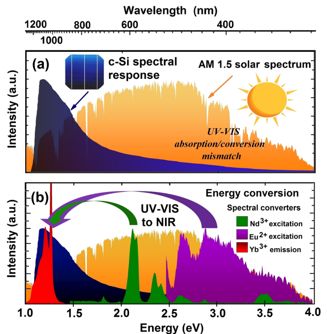
FIG. 5. (a) Orange background is the solar spectrum (AM1.5G) in the UV-Vis-NIR regions. The gray is the spectral response of the c-Si. The spectral mismatch is quite evident. (b) Purple and green curves are the optical absorption coefficients of \text{Eu}^{2+} and \text{Nd}^{3+} activators, and the red curve is the \text{Yb}^{3+} sensitizer emission around 980 nm, close to the c-Si bandgap.
