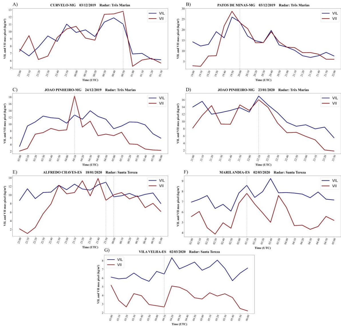
Figure 2. Vertically integrated liquid (VIL) and ice (VII) lifecycle for the highest value pixel for each analyzed event. The dashed vertical line indicates the time of maximum reflectivity value recorded by the rain gauge for each event, here called Pmax.
