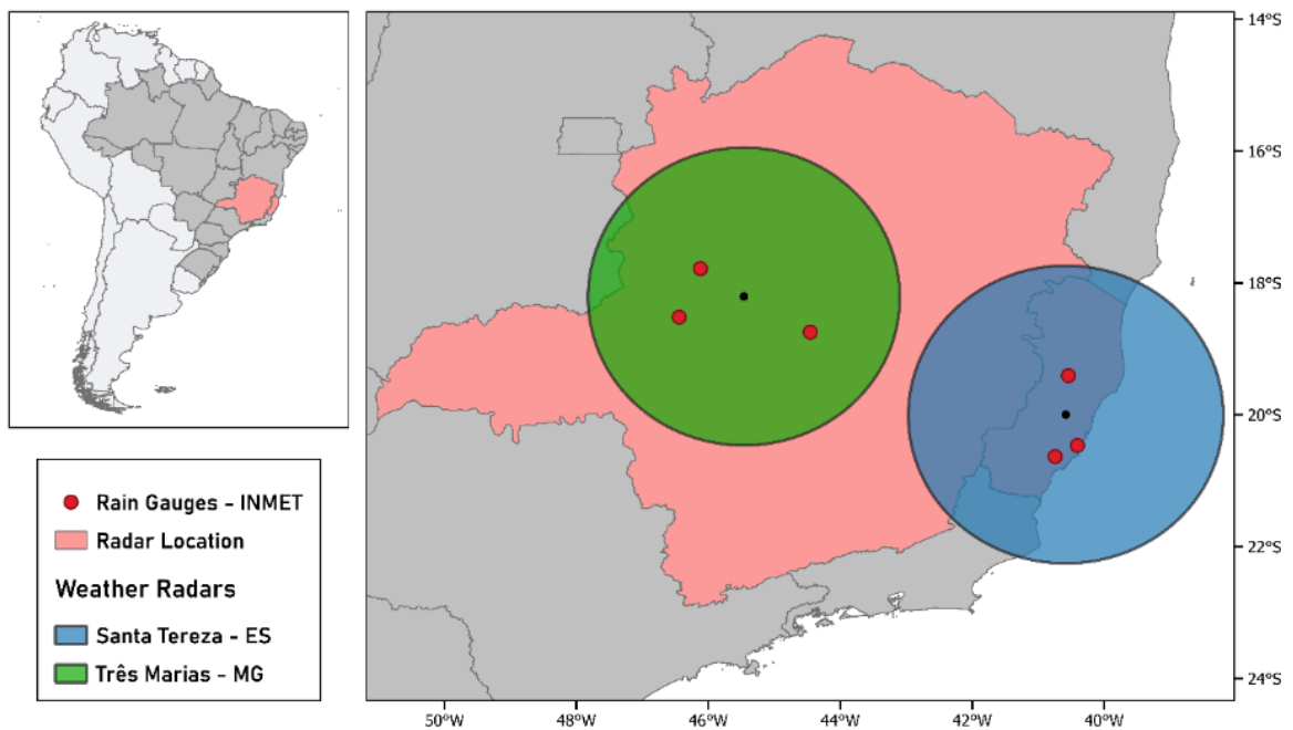
Figure 1 - Location of the Santa Tereza (blue) and Três Marias (green) polarimetric radars and the rain gauges selected for the study.
