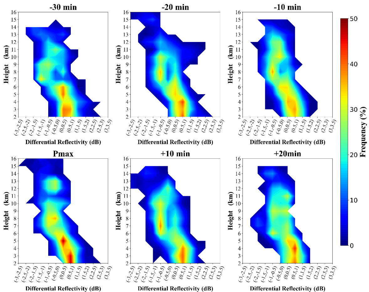
Figure 4. Same as Figure 3, but the x-axis refers to Differential Reflectivity (Zdr) values in dB.
