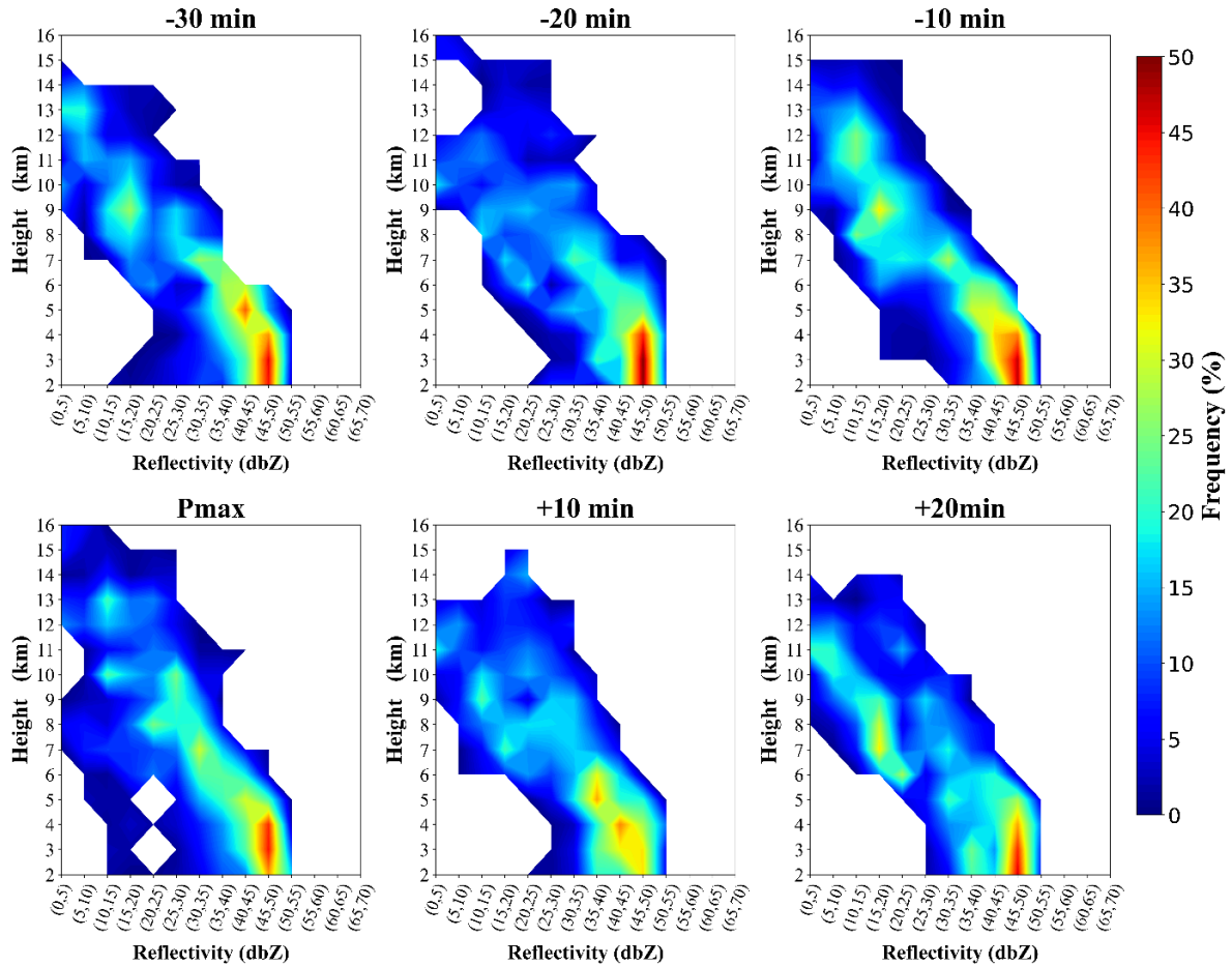
Figure 3. Frequency diagram (CFAD) using a 25 km 2 sample centered on the maximum VIL value for —30, —20, and —10 minutes before the occurrence of the maximum reflectivity value at the location of the rain gauge (Pmax), and +10, +20 minutes after registration. The y-axis refers to height in km and the x-axis to reflectivity intervals in dBZ.
