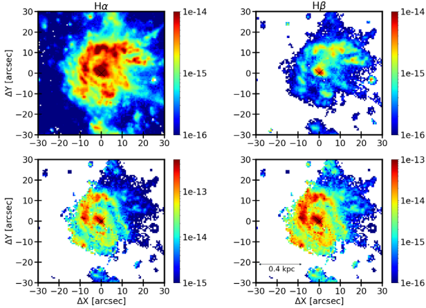
Figure 5. Flux maps for H \alpha (left panels) and H \beta (right panels) before (top) and after (bottom) reddening correction. The colour bar is in units of \text{erg s}^{-1} \text{cm}^{-2} \text{Spaxel}^{-1} . White areas correspond to mask values of SNR < 3. The black cross indicates the AGN position.
