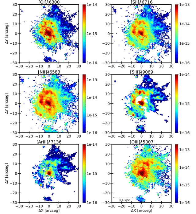
Figure 6. Emission line flux distribution for [O I] \lambda 6300, [S II] \lambda 6716, [N II] \lambda 6583, [S III] \lambda 9069, [Ar III] \lambda 7136, and [O III] \lambda 5007. The colour bar is in units of \text{erg s}^{-1} \text{cm}^{-2} \text{Spaxel}^{-1} . North is up and East to the left.
