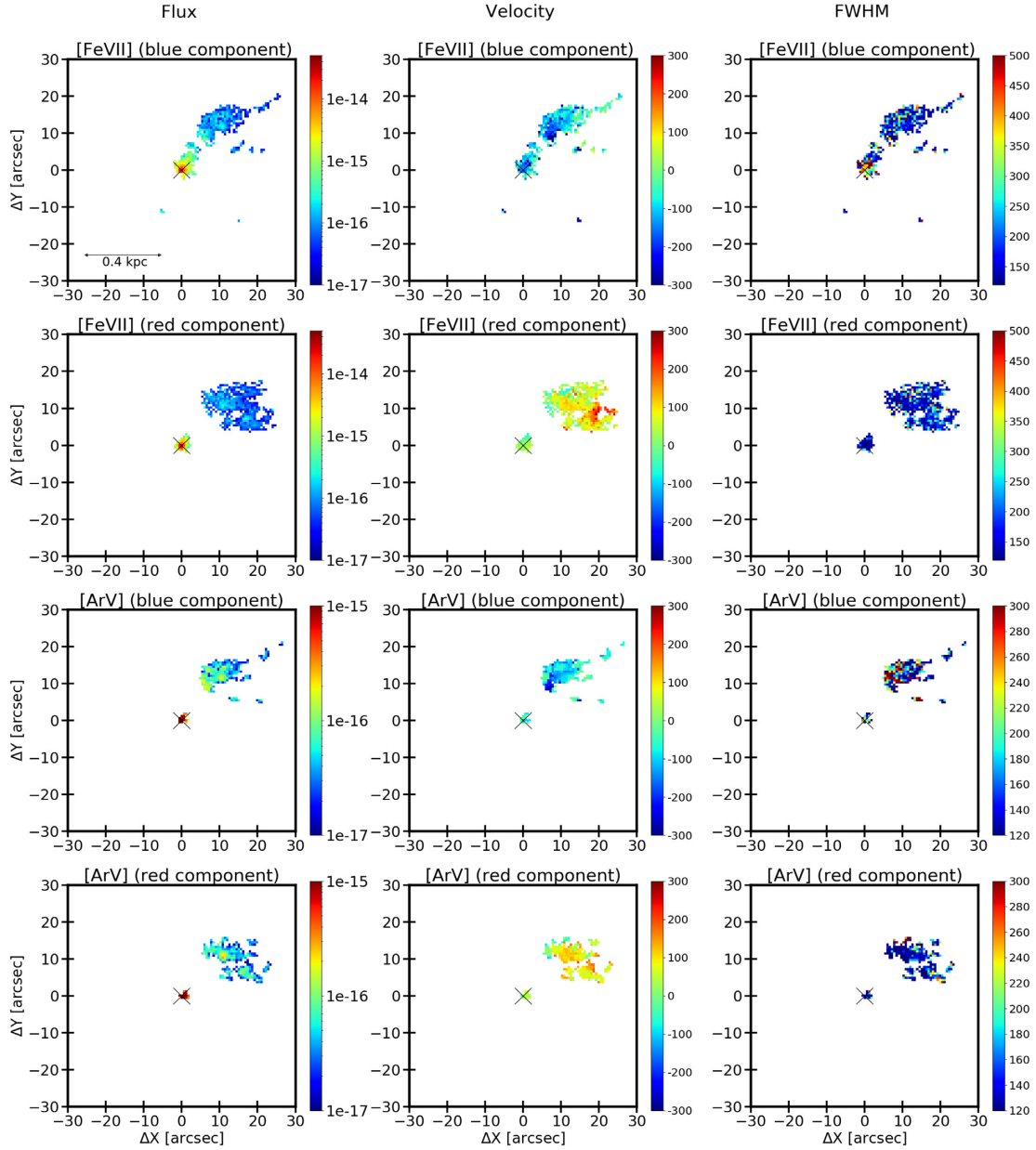
Figure 17. Moment maps for the high-ionization lines [\text{Fe VII}]\lambda 6087 and [\text{Ar V}]\lambda 7006 . Flux scale is in units of \text{erg s}^{-1} \text{cm}^{-2} \text{Spaxel}^{-1} . Velocity and FWHM are in units of \text{km s}^{-1} .
