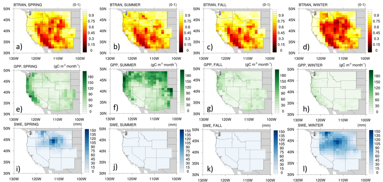
Figure 7. The CLM5-DART (state-13) assimilation average behavior (1998–2010) for (a–d) BTRAN ( \beta_t ), (e–h) gross primary productivity, and (i–l) SWE (snow water equivalent) for meteorological spring, summer, fall, and winter. The \beta_t value is a diagnostic for soil moisture limitation upon GPP with low ( \sim 0 ) and high ( \sim 1 ) values indicating strong and weak limitation, respectively.
