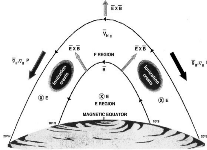
Figure 2.5 - The formation of Equatorial Ionization Anomaly is driven mainly from the removal of plasma from around the equator by the upward E \times B drift creating the trough and consequently the crests with small accumulation of plasma within \pm 20^\circ magnetic latitudes, as depicted by (MATHIS, 2013).
