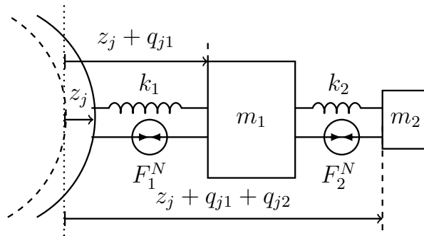
Figure 3.2 - Body diagram of a system of a two mode resonant transducer coupled to the surface of a vibrating sphere.
