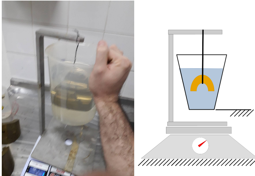
Figure 5.2 - Picture and diagram of the process for determining density. A sample of the CuAl alloy was suspended from a wire of negligible mass and volume, connected to a frame that sits atop a scale. As a bucket of water is inserted beneath then submerges the sample, the scale should register the weight of displaced liquid.
