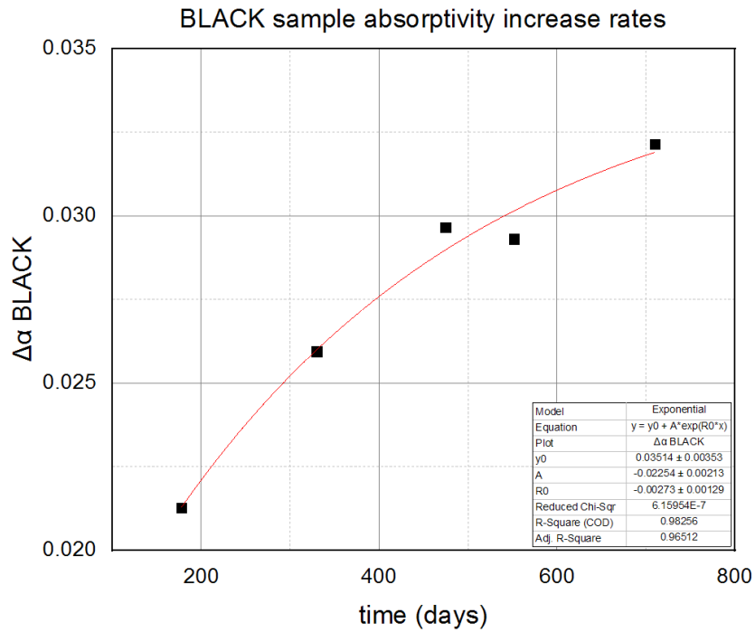
Figure 10.27 – Degradation of the solar absorptivity for Black Anodized.
