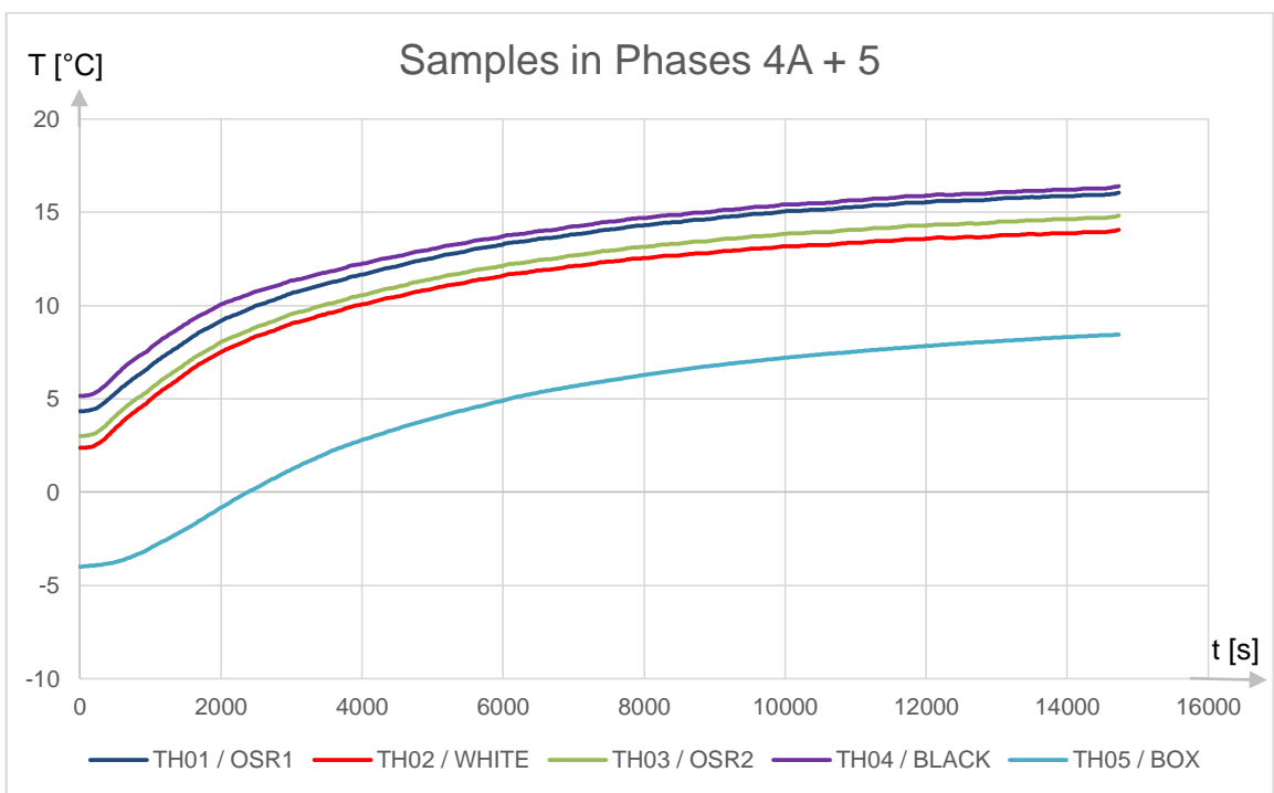
Figure G.2 – Corrected Experiment Therm. TBT Temperatures for 4A and 5.
