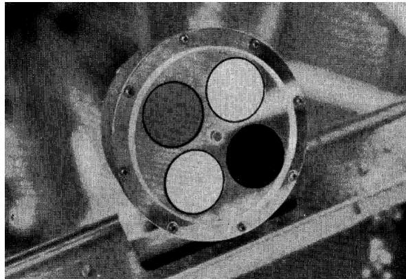
Figure 1.7 – Pegasus Thermal Control Coatings Experiment Package.
