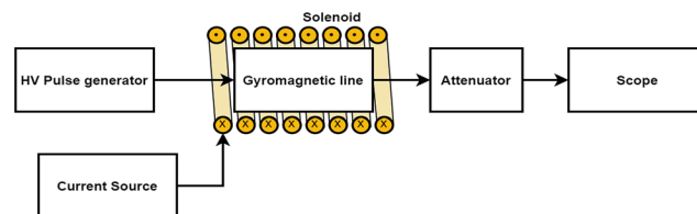
FIG. 3. Block diagram of the experimental setup used to test the GNLTL.
