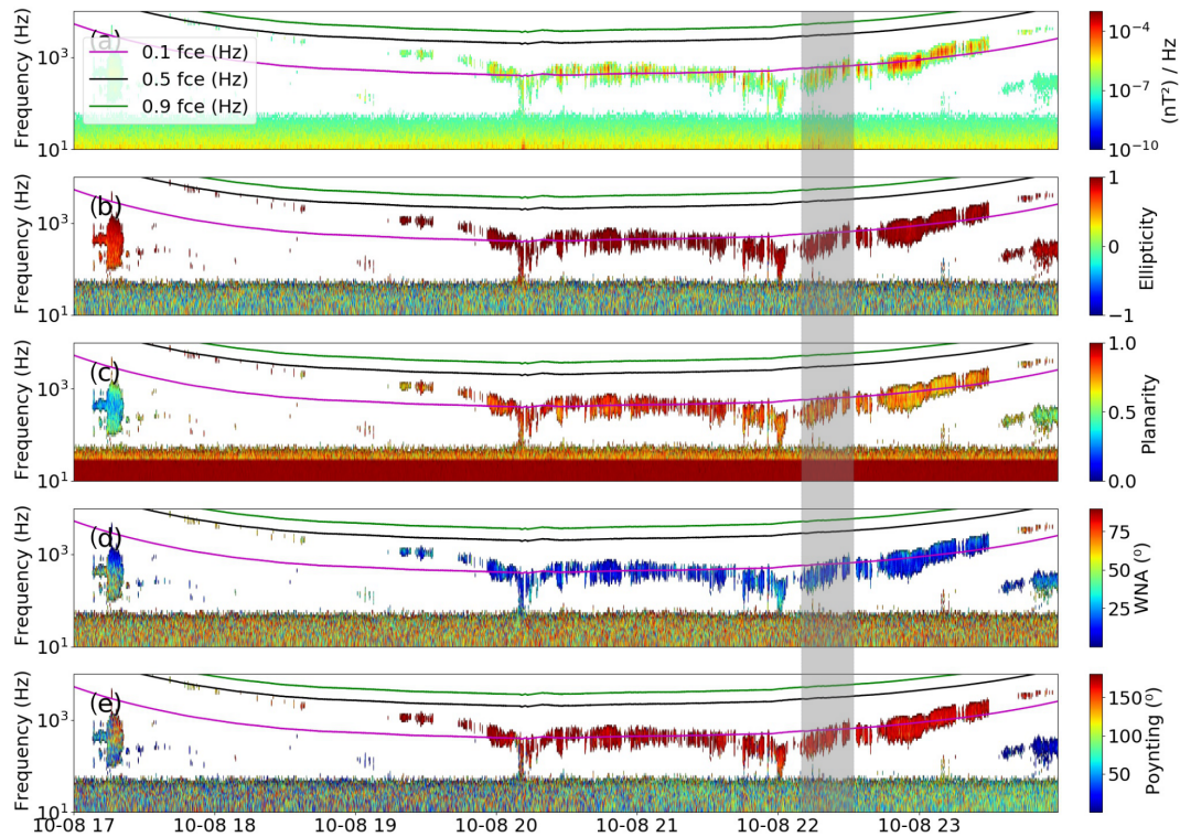
Figure 6. Case 1. Panels show the whistler-mode chorus waves' (a) spectrum of the magnetic field, (b) ellipticity, (c) planarity, (d) WNA (wave normal angle), and (e) the polar angle of the Poynting vector. In all panels, the values of 0.1 fce (electron cyclotron frequency) (Hz), 0.5 fce (Hz), and 0.9 fce (Hz) are shown by the pink, black, and green lines, respectively. The parameters shown by the shaded region were used to calculate the interaction time, change in pitch angle, and diffusion coefficient for the resonant electrons energy shown in Table 1.
