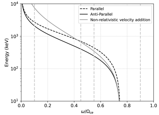
Figure 2. Comparison of the electron resonant kinetic energy (keV) as a function of whistler-mode chorus wave frequency normalized by the electron gyrofrequency propagating parallel and antiparallel to the ambient magnetic field ( B_0 = 150 nT). The wave–particle resonance condition depends on the wave dispersion relation ( \omega/k ), calculated from Eq. (2), with n = +5 . The vertical lines delimitate the low-band whistler-mode chorus wave frequency corresponding to 0.1 f_{ce} \leq f \leq 0.45 f_{ce} and the high-band 0.55 f_{ce} \leq f \leq 0.90 f_{ce} as a fraction of the electron gyrofrequency. Plasma parameters are the same as those used in Fig. 1.
