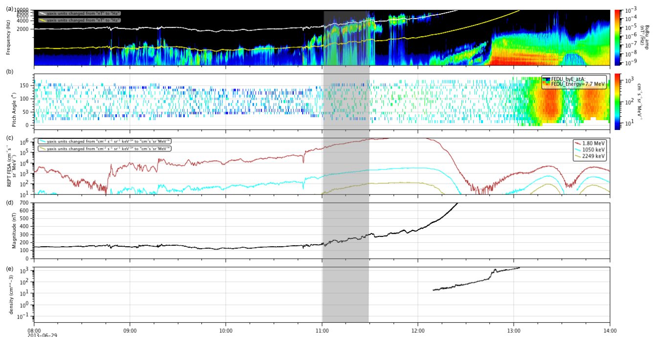
Figure A1. Case 2. Panels show from (a) to (e) the whistler-mode chorus waves' spectrum, the interpolated 1.8 MeV electron flux pitch angle distribution, the relativistic and low-energy electron fluxes, the ambient magnetic field, and the local plasma density for the whistler-mode chorus waves observed on 29 June 2013. The parameters shown in the highlighted area were used to calculate the time of interaction and change in pitch angle for the energy of the resonant electrons shown in Table 1.
