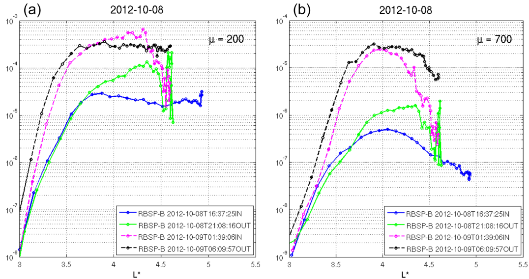
Figure 7. Case 1. Time evolution of phase space density (PSD [ c/(\text{cm MeV})^3 \text{sr}^{-1} ]) radial profiles at fixed first adiabatic invariant, \mu = 200 \text{ MeV G}^{-1} (a) and \mu = 700 \text{ MeV G}^{-1} (b), and second ( K = 0.11 G^{1/2} R_E ) adiabatic invariant for both inbound and outbound parts of the RBSP-B orbit. Period of analysis: 8 October 2012 from 16:37 UT through the interval of interest.
