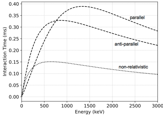
Figure 4. Comparison of time of interaction (ms) as a function of electron resonant kinetic energy (keV) calculated using Eq. (13) (dashed lines) and the non-relativistic approach (dotted line) for parallel and antiparallel wave propagation. Plasma parameters are B_{\text{am}} = 166 nT, \tau = 1.8 ms, and n_e = 3.0 \text{ cm}^{-3} .
