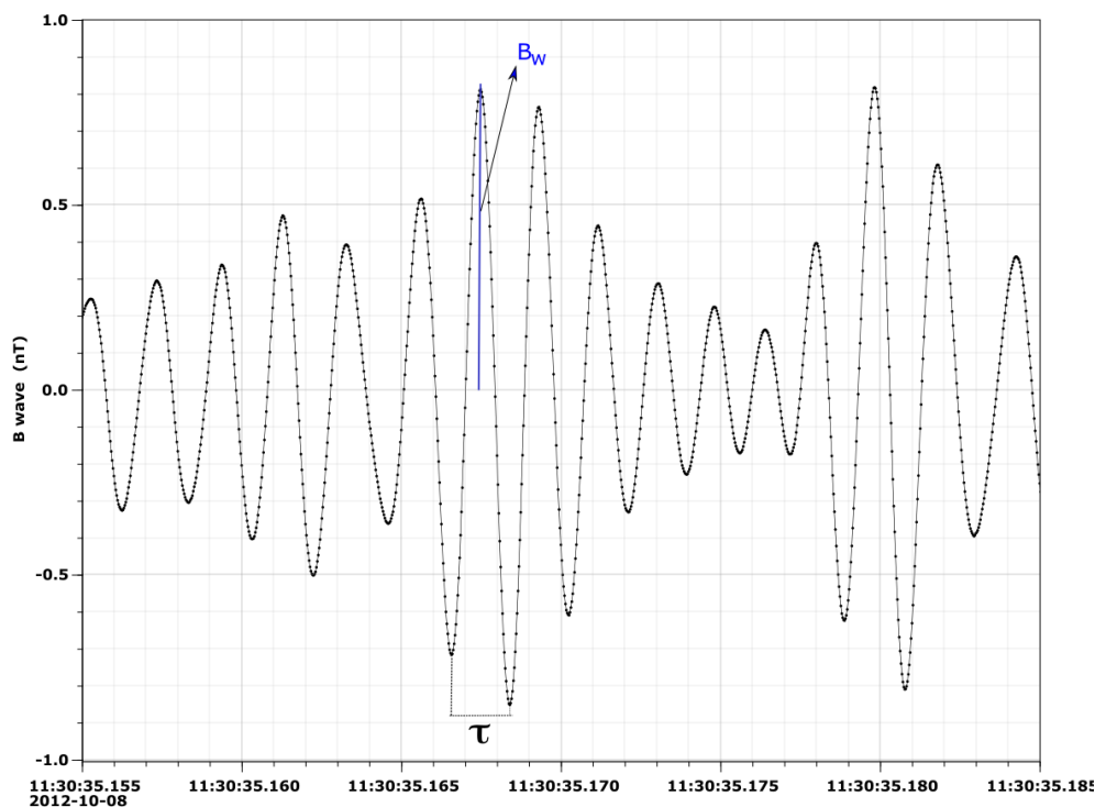
Figure G1. The high-resolution magnetic field measurement related to the event on 8 October 2012. A similar plot was made for the other three studied events. The figure identifies the maximum instantaneous wave magnetic field amplitude B_w and the one wave cycle period \tau .
