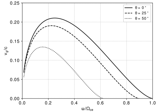
Figure 1. Group velocity v_g/c as a function of whistler-mode chorus wave frequency to the plasma gyrofrequency for the propagation of three different wave normal angles. This group velocity is the full solution of Appleton–Hartree for whistler waves propagating in low-density plasma media at any orientation. The Van Allen Probes apogee orbit provides plasma parameters used in the calculation, B_0 = 150 \text{ nT} and low density n = 2 \text{ cm}^{-3} .
