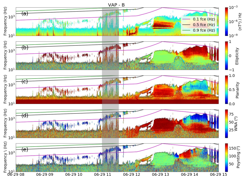
Figure B1. Case 2. Panels from 29 June 2013 show the whistler-mode chorus waves' (a) spectrum of the magnetic field, (b) ellipticity, (c) planarity, (d) WNA (wave normal angle) and (e) the polar angle of the Poynting vector. In all panels, the values of 0.1 fce (Hz), 0.5 fce (Hz), and 0.9 fce (Hz) are shown by the pink, black, and green lines, respectively. The parameters shown from the gray-shaded period are used to calculate the time of interaction and change in pitch angle for the resonant electrons energy shown in Table 1.
