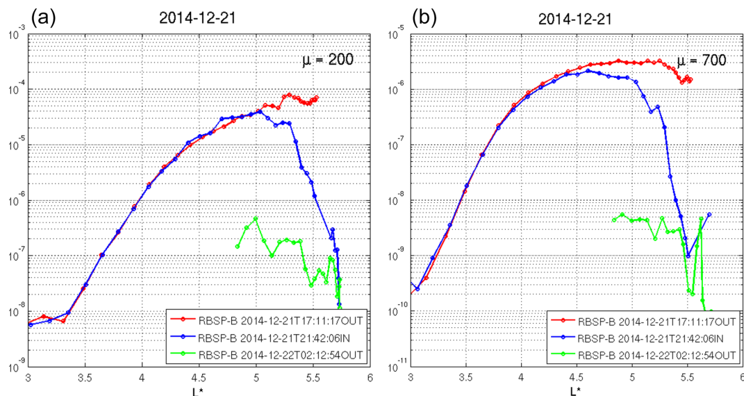
Figure F1. Same as Fig. C1 but for both inbound and outbound parts of the RBSP-B orbit in the period of analyses: 21 December 2014 at 17:11:17 UT to 22 December 2014 at 02:12:54 UT.
