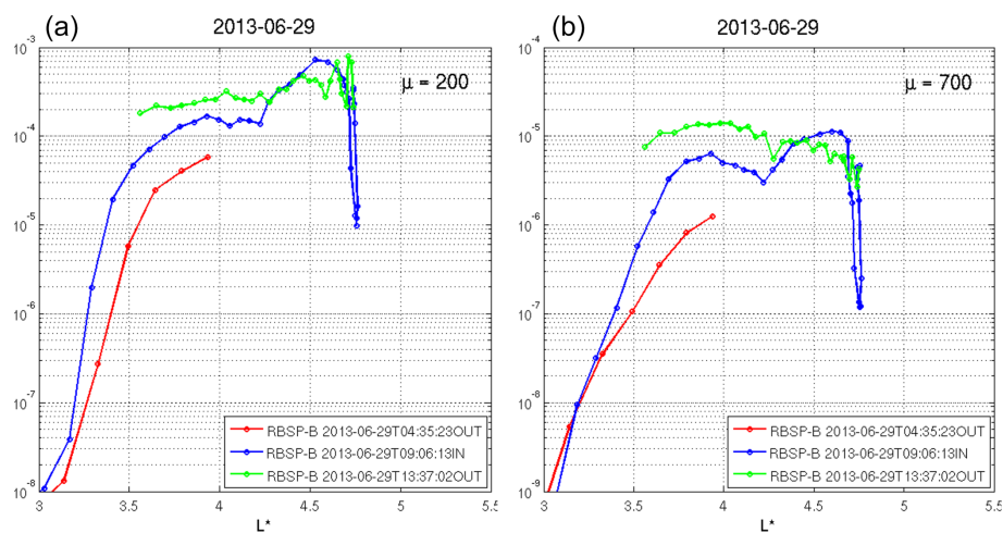
Figure C1. Case 2. Time evolution of phase space density (PSD) radial profiles at fixed first adiabatic invariant, \mu = 200 \text{ MeV G}^{-1} (a) and \mu = 700 \text{ MeV G}^{-1} (b), and second ( K = 0.11 G^{1/2} R_E ) adiabatic invariant for both inbound and outbound parts of the RBSP-B orbit. Period of analyses: 29 June 2013 at 04:35:23 to 13:37:02 UT.
