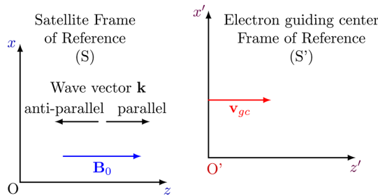
Figure 3. Illustration of the two reference frames used in calculating the interaction time in Sect. 3. The electron guiding center frame of reference ( S' ) has a velocity \mathbf{v}_{gc} with respect to the satellite frame of reference ( S ). This velocity parallels the ambient magnetic field \mathbf{B}_0 . Thus, the angle between the wave vector \mathbf{k} and \mathbf{v}_{gc} equals the WNA, and it is 0^\circ for parallel and 180^\circ for antiparallel propagating waves.
