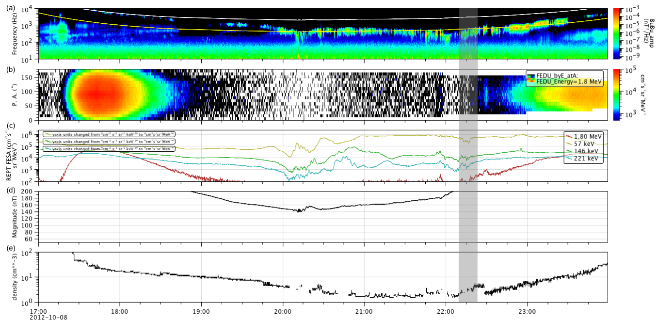
Figure 5. Case 1. Panels show from (a) to (e) the whistler-mode chorus waves' spectrum, the interpolated 1.8 MeV electron flux pitch angle distribution, the relativistic and low-energy electron fluxes, the ambient magnetic field, and the local plasma density. The parameters shown in the shaded region were used to calculate the interaction time, change in pitch angle, and diffusion coefficient for the resonant electrons energy shown in Table 1.
