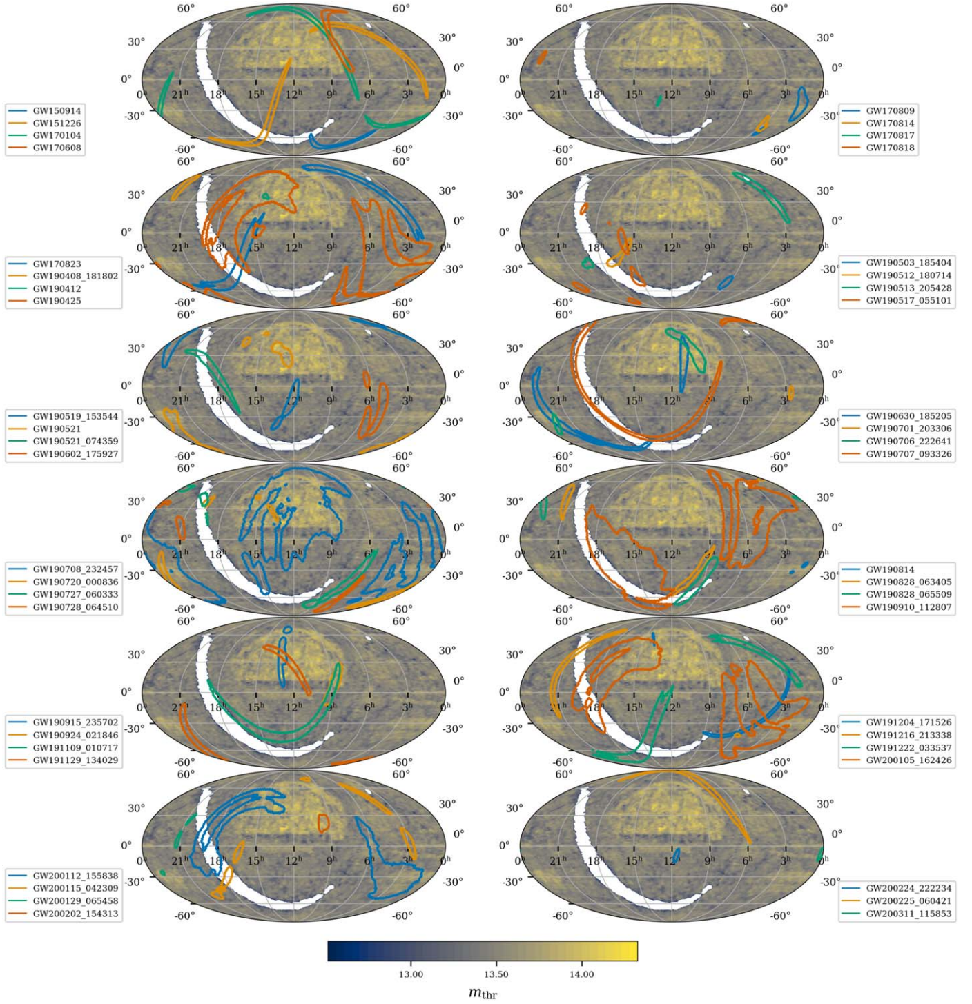
Figure 2. Sky maps showing the GLADE+ K -band apparent magnitude threshold, m_{\text{thr}} , generated by dividing the sky into 3.35 \text{ deg}^2 pixels; this is the resolution used for all the events but GW190814. A mask is applied that removes from the figures all pixels with m_{\text{thr}} < 12.5 in order to improve the figure readability. Also shown are the 90% CL sky localizations for the GW events considered in this paper.
