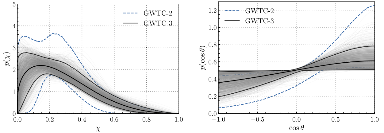
FIG. 15. The distributions of component spin magnitudes \chi (left) and spin-orbit misalignment angles \theta (right) among binary black hole mergers, inferred using the DEFAULT component spin model described further in Sec. 2 a; e.g., both spin magnitudes are drawn from the same distribution. In each figure, solid black lines denote the median and central 90% credible bounds inferred on p(\chi) and p(\cos \theta) using GWTC-3. The light gray traces show individual draws from our posterior distribution on the DEFAULT model parameters, while the blue traces show our previously published results obtained using GWTC-2. As with GWTC-2, in GWTC-3 we conclude that the spin-magnitude distribution peaks at \chi_i = 0.13^{+0.12}_{-0.11} , with a tail extending toward larger values. Meanwhile, we now more strongly favor isotropy, obtaining a broad \cos \theta_i distribution that may peak at alignment ( \cos \theta_i = 1 ) but that is otherwise largely uniform across all \cos \theta .
