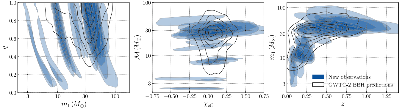
FIG. 1. New observations since GWTC-2. The measured properties of new CBC candidates announced since GWTC-2 with FAR < \text{yr}^{-1} and reported parameters (blue shaded regions) compared to the expected population of detected BBHs (black contours) as inferred from past analysis of GWTC-2 with the same FAR threshold [114] and the fiducial binary parameter priors described in the text. The left-hand plot shows the inferred primary mass m_1 and mass ratio q , the center plot shows the effective spin \chi_{\text{eff}} and chirp mass \mathcal{M} , and the right plot shows redshift z and primary mass. The least-massive sources in this sample include NSBH events GW200105 and GW200115.
