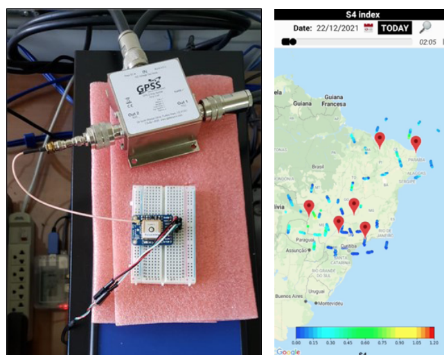
Figure 6. Future instrumentation trend, low-cost scintillation monitors. Left panel: GPS module Adafruit Ultimate GPS Breakout. Right panel: ScintApp screen showing the Brazilian map with the available stations during a proof-of-concept experiment and their respective ionospheric pierce points. The bar indicating the strength of scintillation is shown at the bottom of the app screen.
