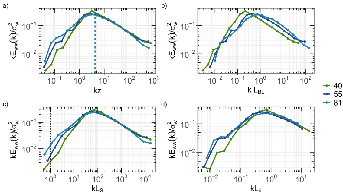
FIG. 4. Pre-multiplied normalized vertical velocity spectra, k E_{wv}(k)/\sigma_w^2 at different heights for ATTO as reference. Panel (a) shows the spectra as a function of kz . Panels (b), (c), and (d), represent k normalized using kL_{BL} , kL_s and kL_d , respectively. The vertical dashed lines refer to: in panel (a), k_a estimates at the different heights; in panels (b)–(d), kL_\chi = 1 , where L_\chi = L_{BL} , L_s , and L_d . Note the collapse of the spectral peaks at kL_d = 1 for all z/h in panel (d).
