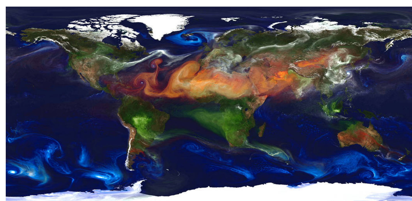
High-resolution global atmospheric modeling run of the NASA Center for Climate Simulation, Goddard Earth Observing System Model, Version 5 (GEOS-5). 10km Global aerosols simulation. Dust (red), sea salt (blue), smoke (green), and sulfate particles (white). Source: https://www.nasa.gov/multimedia/imagegallery/image_feature_2393.html
