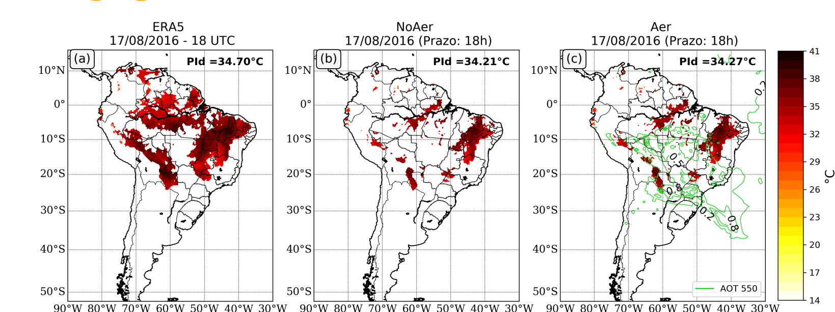
NWP experiment: ECMWF-IFS heatwave forecast considering the experiment INT and experiment NOINT .
