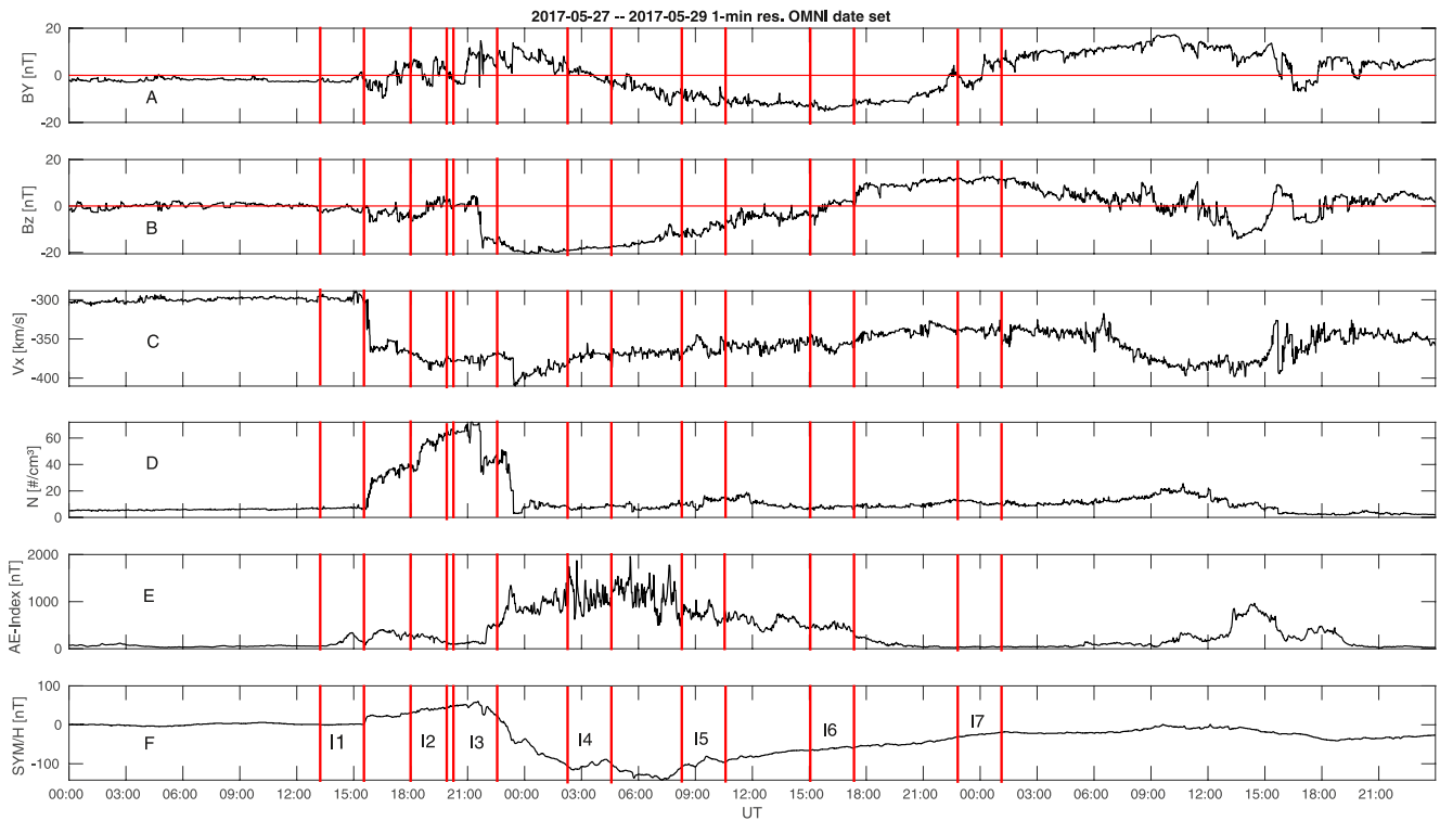
Figure A1. Shows solar wind plasma parameters AE and SYM-H magnetospheric indices. The vertical red lines represent each 2 hr long I's interval. Panels (a–d) illustrate the B_y , B_z , V_x and the solar wind density respectively. Panels (e, f) show the AE and SYM-H indices that illustrate the activity level of the inner magnetosphere. The data obtained in: https://omniweb.gsfc.nasa.gov/form/omni_min.html .
