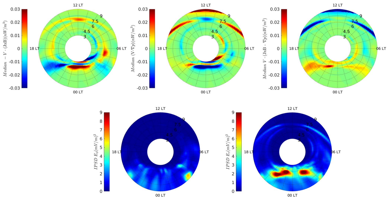
Figure 8. Represents the I_2 interval. The first row above left to right represents the median of the magnetic energy conversion term, the second represents the internal energy conversion term and the last term represents the kinetic energy conversion. The second row represents the integrated power spectral density of the azimuthal and radial electric field component in the equatorial plane at z = 0 . Both the median and the integrated values were taken within 2 hr long.
