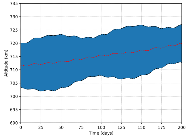
Fig. 8. Spacecraft's altitude as function of time for Strategy 2. The color figure can be viewed online.
