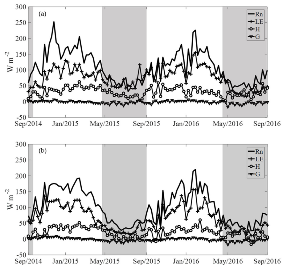
Figure 4. Weekly average of the energy balance components: net radiation, Rn ( W m^{-2} ); sensible heat flux, H ( W m^{-2} ); latent heat flux, LE ( W m^{-2} ); and soil heat flux, G ( W m^{-2} ) from 1 September 2014 to 1 September 2016, for the Pampa biome, at the (a) SMA and (b) PAS sites. The points represent the average every six days. The hatched areas represent the autumn-winter (AW) periods.
